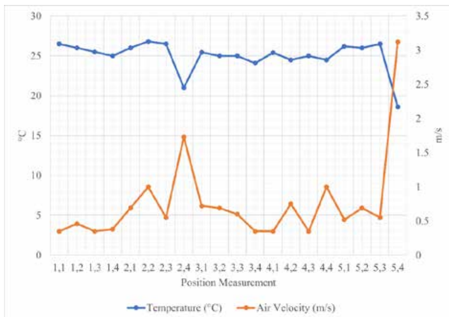
Figure 6. Chart of Results Temperature and Air Velocity at Lecture Room BK 31 After CFD Simulation for Actual Application
