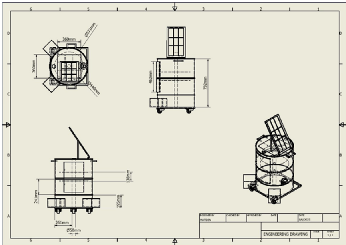
Figure 2 Design of the solar food dehydrator.
