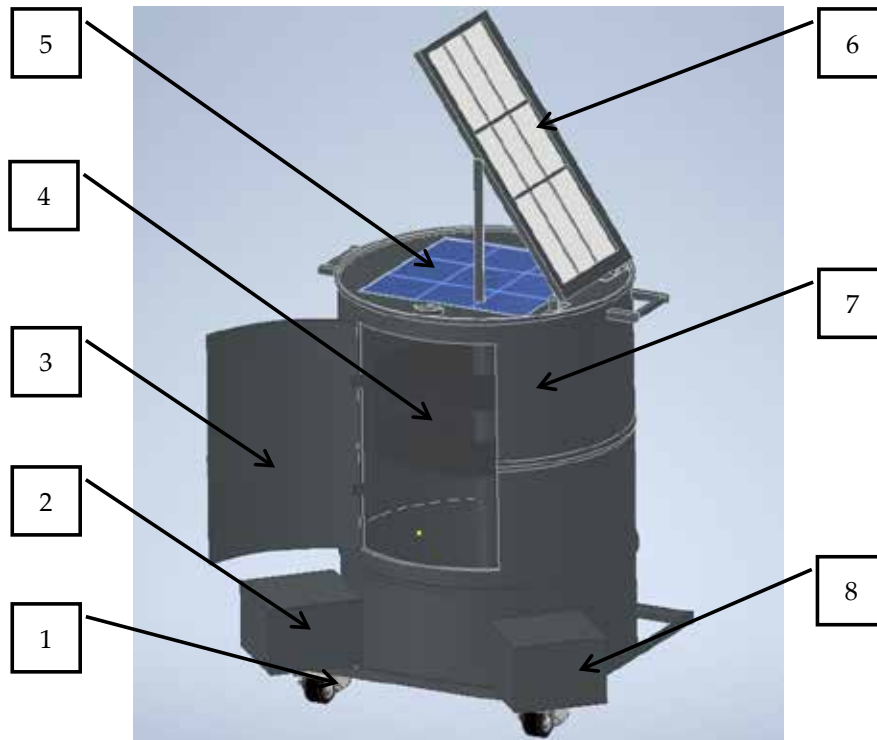
Figure 3: the overall structure after completely assembly of the solar food dehydrator
