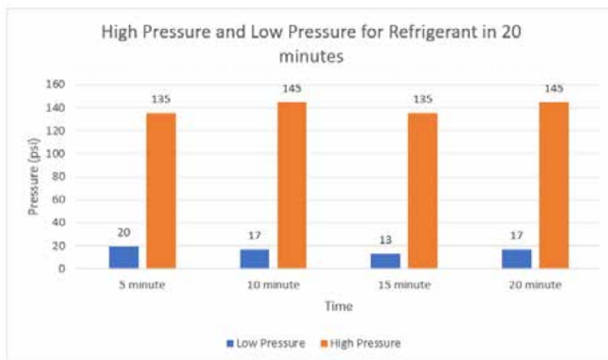
Figure 4. Result of high pressure and low pressure for refrigerant in 20 minutes
