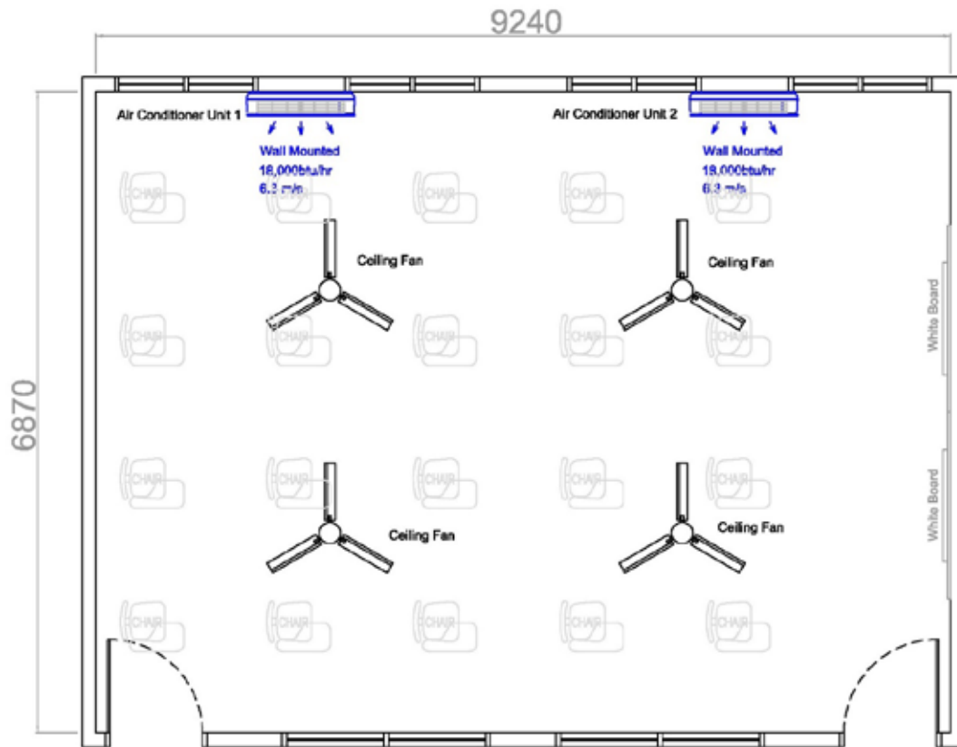
Figure 2. Geometry of Lecture Room Equipped with Ceiling Fans and Wall Mounted Split Unit Air-Conditioner.
