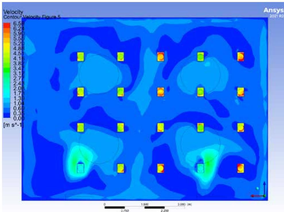
Figure 5. Contour Air Velocity on Plane X elevation 1500 mm
