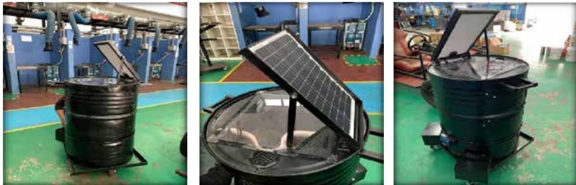
Figure 5: Installation of solar panel, battery and test run of system
