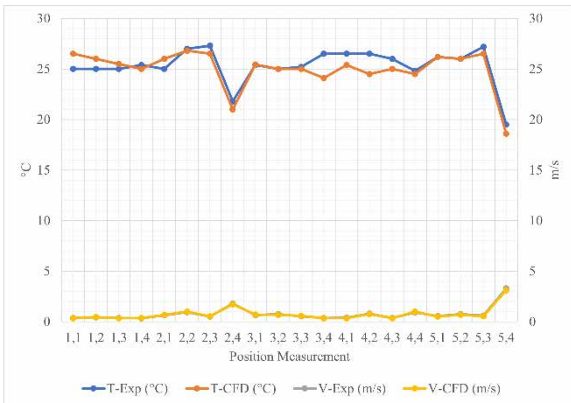
Figure 7. Chart of Temperature and Air Velocity for the Experiment and CFD Simulation on Actual Lecture Room
