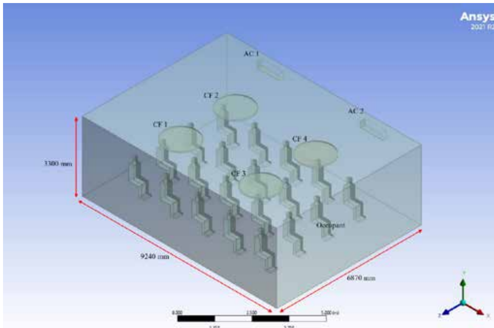
Figure 3. The BK 31 Geometry Design Modeler Base on Actual Condition
